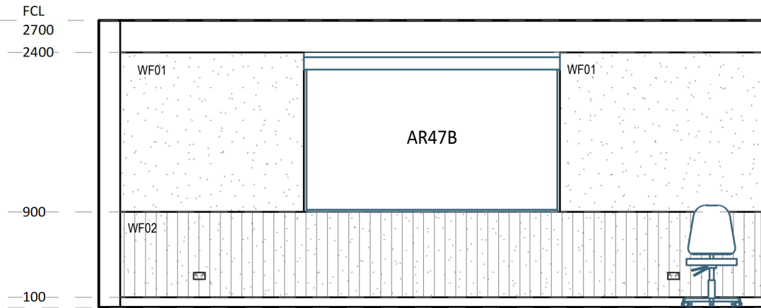
3 ELEVATION DETAIL 1 : 50
