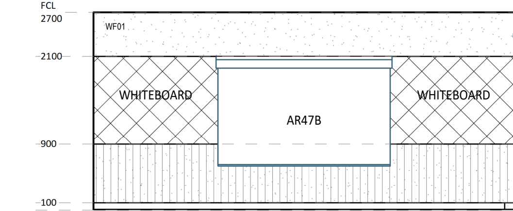
7 ELEVATION DETAIL 1 : 50
