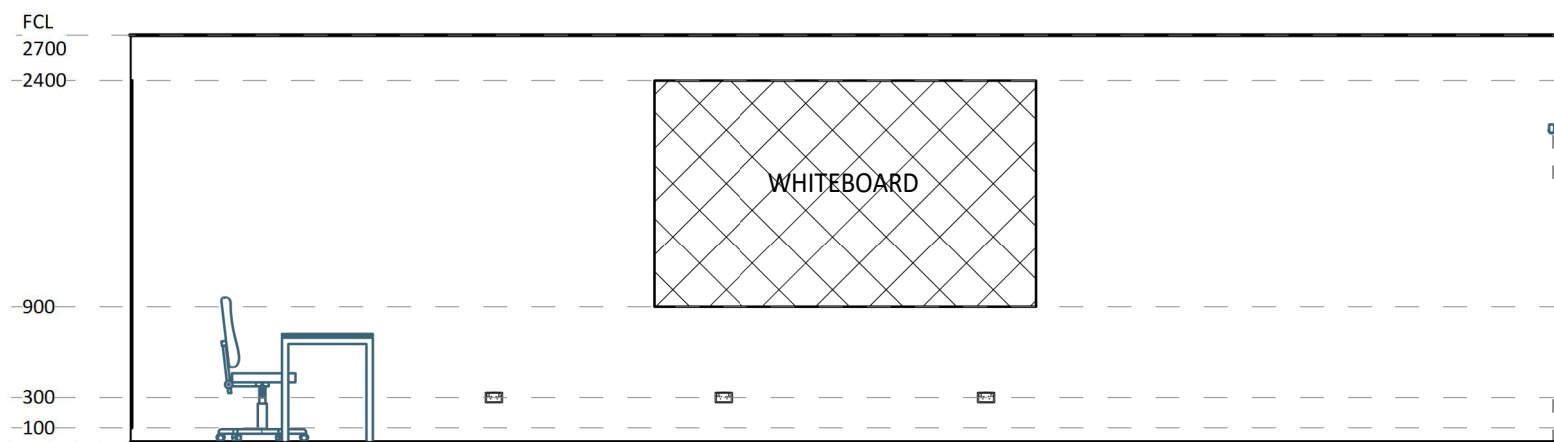
9 ELEVATION DETAIL 1 : 50
