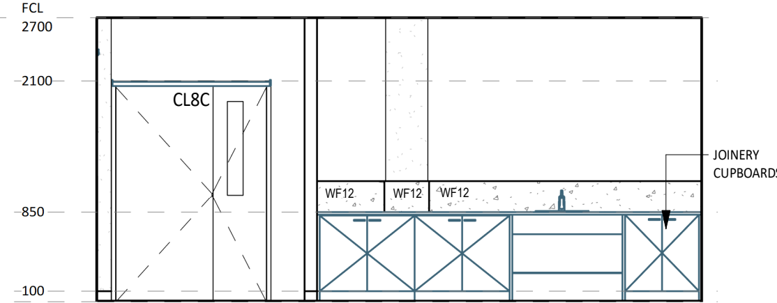
8 ELEVATION DETAIL 1 : 50
